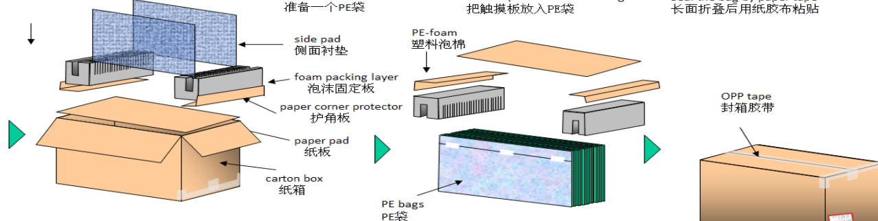
Prepare a touch panel 准备触摸板
