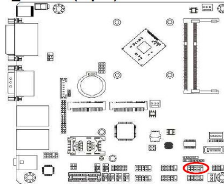
(5) FP_USB20 (9-pin): USB 2.0 Port Header
